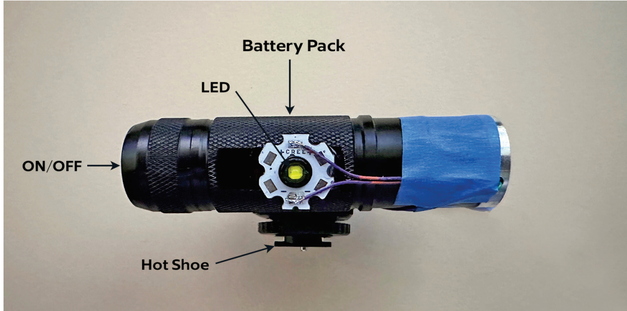
A prototype Macro focusing light—front view.
